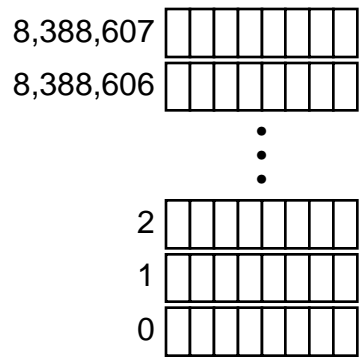
Figure 7.2 Addressing scheme for 8 megabytes of bytes.
