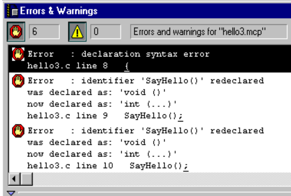
Figure 4.9 Yikes! All this just because you added a single semicolon!
