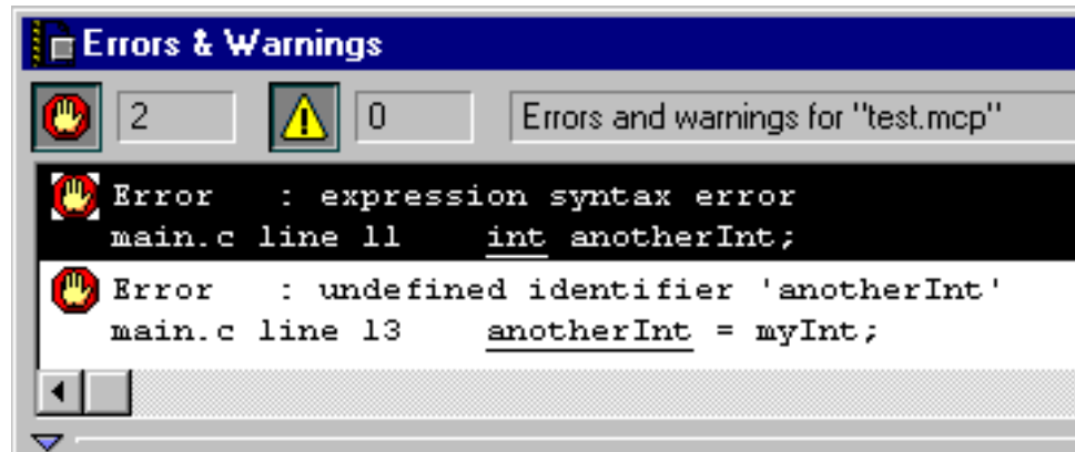
Figure 5.6 These errors occurred because anotherInt was declared after an assignment statement.
