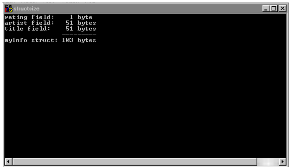
Figure 9.3 structSize shows the size of a CDInfo struct.
