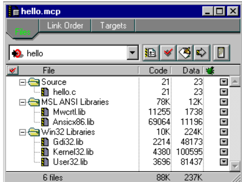
Figure 3.4 The updated project window.
