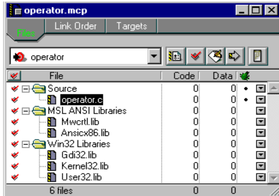
Figure 5.8 The operator .mcp project window.
